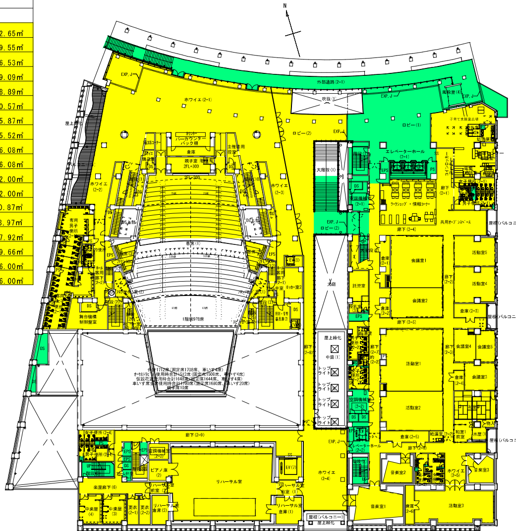
2階平面図 Scale:1/500
